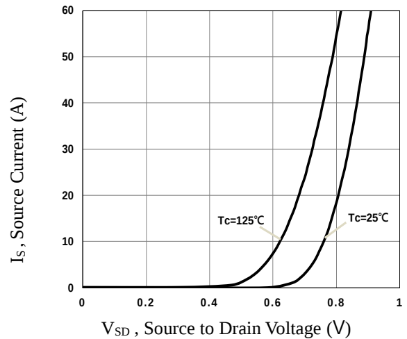
Fig.10 Source Current vs. V_{SD}
