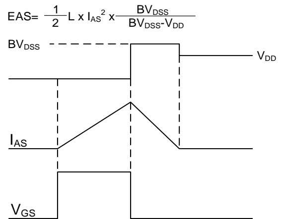
Fig.12 EAS Waveform
