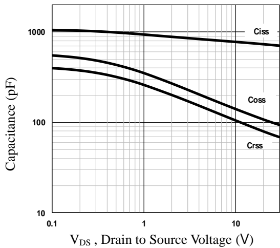
Fig.5 Capacitance Characteristics
