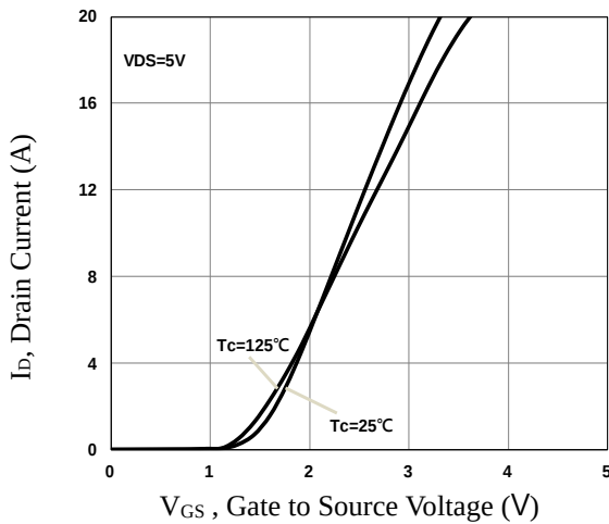
Fig.9 Transfer Characteristics
