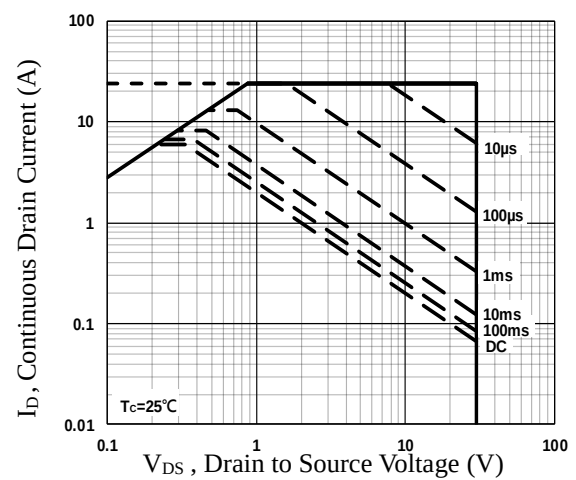
Fig.11 Maximum Safe Operation Area
