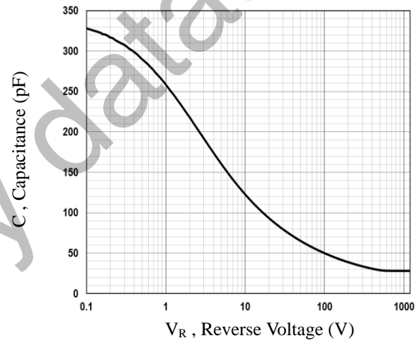
Fig.4 Capacitance Characteristics
