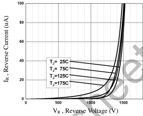
Fig.2 Reverse Characteristics
