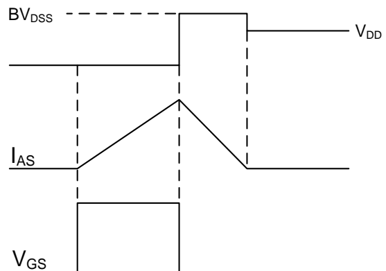
Fig.11 EAS Waveform
