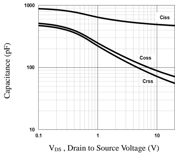
Fig.6 Capacitance Characteristics
