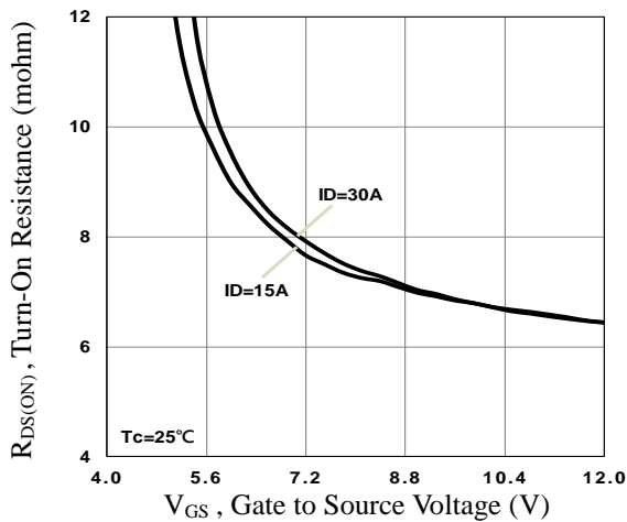
Fig.5 Turn-On Resistance vs. V_{GS}
