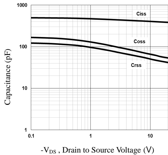
Fig.6 Capacitance Characteristics
