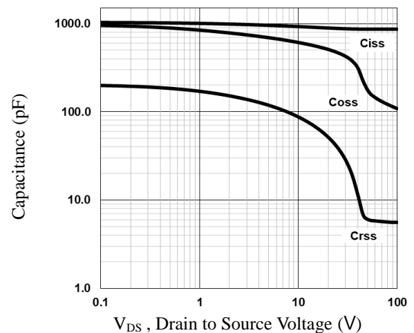
Fig.6 Capacitance Characteristics
