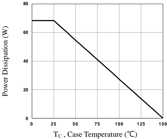
Fig.9 Power Dissipation vs. T_c
